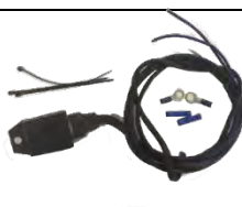
Universal Reg/Rect Kit 12V Regulated to 13.8V COL For use on Outboards with under flywheel lighting coil Instructions Included Part No: RR007CK
