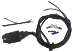
Universal Reg/Rect Kit 12V Regulate to 13.8V CO For use on Outboard with universal fuel lighting oil Instructions include Part No: RR007CK
