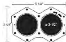
Head Gasket 90° V6 Crossflow (76-91) With a 3.500" Piston
