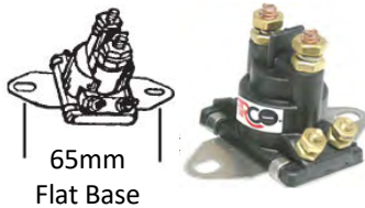
Starter Solenoid Part No: 25661
