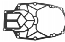
Base Gasket 3.0L Replaces 27-813932 2 Part No: 27-832933 5
