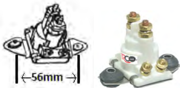
Starter Relay Various 4 stroke 25-40 hp Replaces: 65W-81941-00, 89-850187T1 Part No: 89-818997T1
