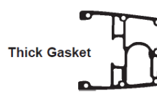
Thick Gasket Powerhead 3 Cyl Mounting Gasket Replaces: 313763 Part No: 328618
