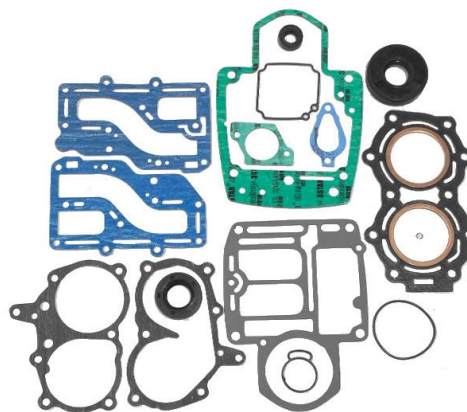
Tohatsu Gasket Set M9.9D2, M15D2 2002-03 Bore 55mm Part No: 3G2-87121-7
