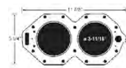
Head Gasket 90° V6 Loopcharged With a 3.6875" Piston (88-92)
